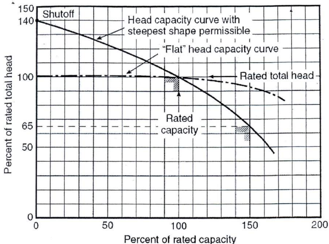
Figure 9.4.1.4 Pump Curve NFPA 20
